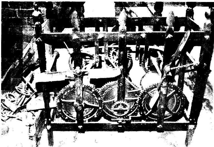
Figure 4. John Eberman's three-train movement for the Nazareth, PA, Moravian Church. If the wheel lying loose in the lower left-hand corner of the photograph is part of this movement, the clock was quarter-hour striking.
