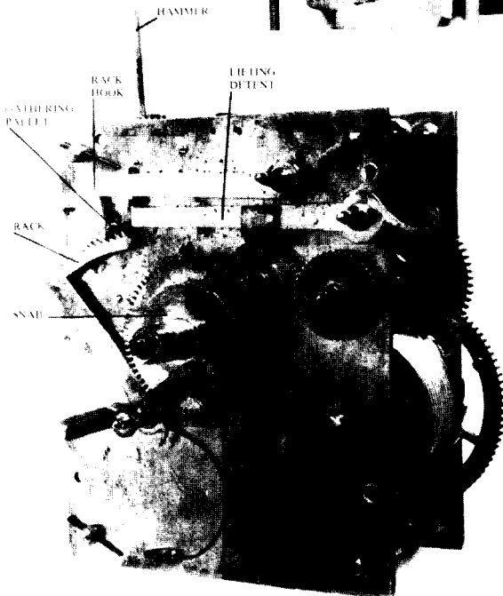
Figure 9. Typical Pennsylvania-German tradition brass 8-day movement. (Private collection)
