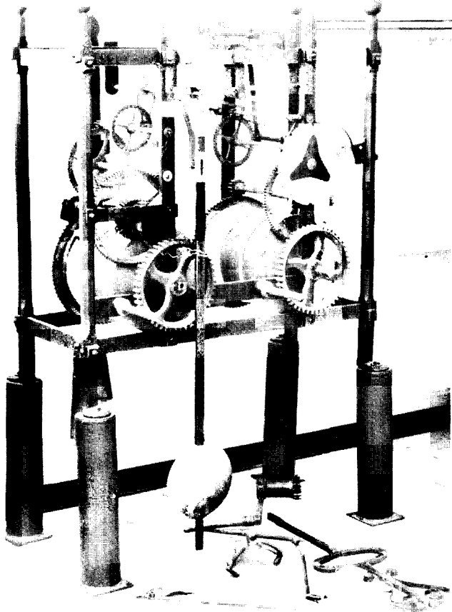
Figure 4. John Eberman's three-train movement for the Nazareth, PA, Moravian Church. If the wheel lying loose in the lower left-hand corner of the photograph is part of this movement, the clock was quarter-hour striking.
