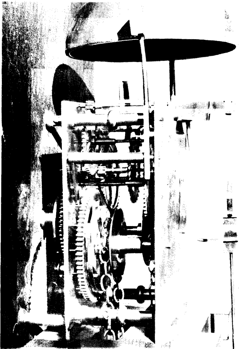
Figure 19. Joseph Eberman 30-hour movement in German tradition. (Private collection)
